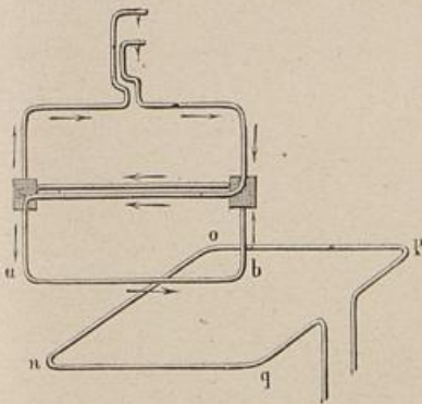
Fig. 2. Astaticer Strom.
