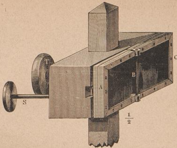
Fig. 1. Fresnel's Spiegelapparat.
