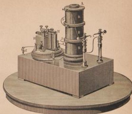
Fig. 3. Edison's Inductor.
