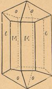
2. Combination von: Brachypyrisma (e) Pyramide (o) Prisma (M). (Topas).
