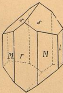
6. Combination von: Orthopyramid (r), Clinopyramid (l), Prisma (M), positive Hemipyramide (s). (Augit.)
