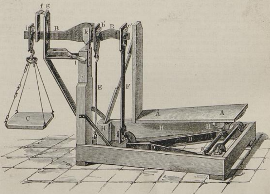
Fig. 3. Decimalwage.
